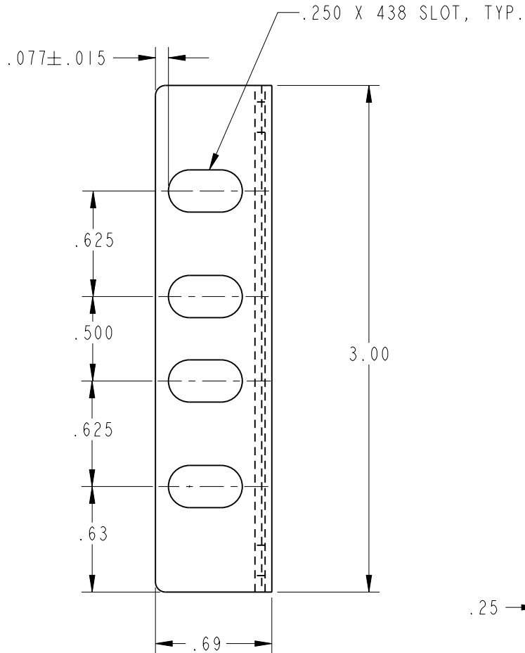
TYPICAL END VIEW
