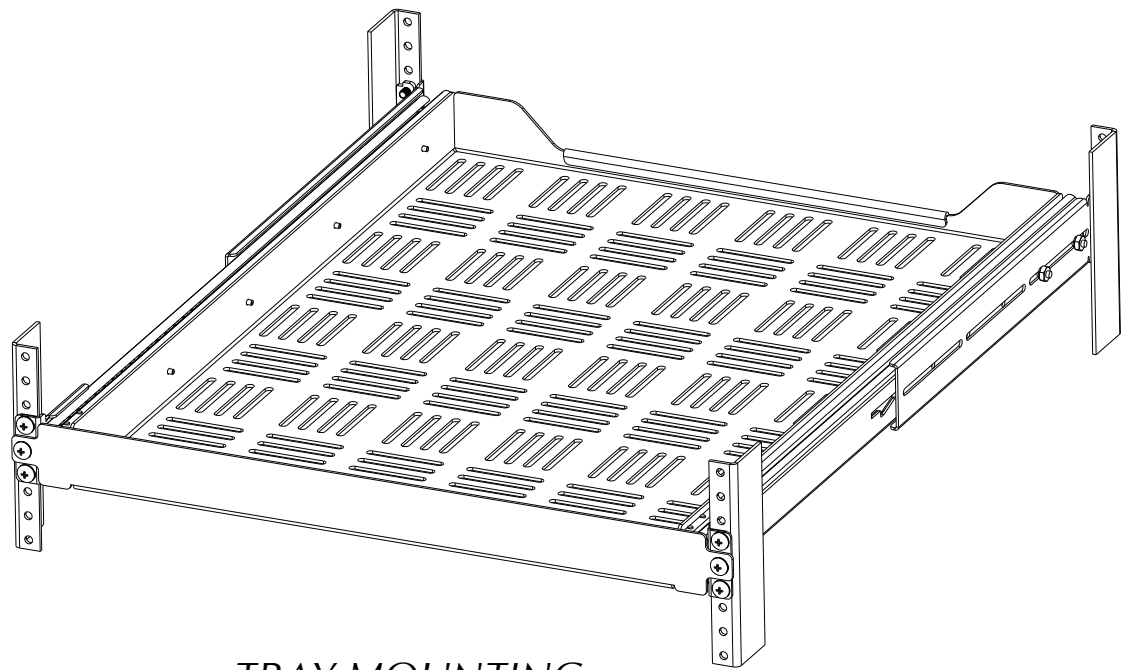
TRAY MOUNTING
