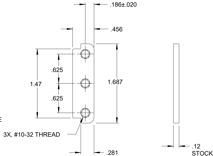
BAR NUT PART NO.: SPO-623
