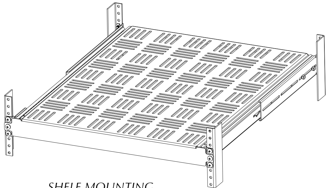
SHELF MOUNTING
