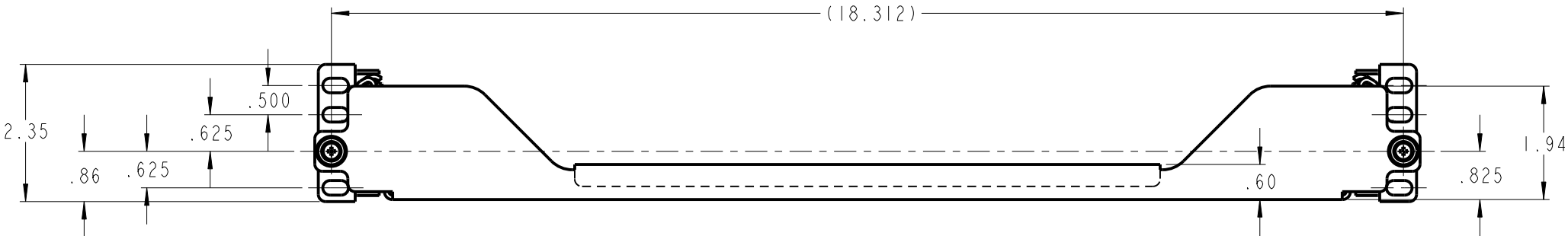
FRONT VIEW
